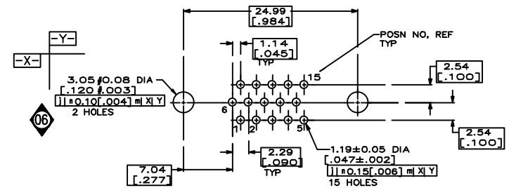
P.C. BOARD MOUNTING DIMENSIONS
